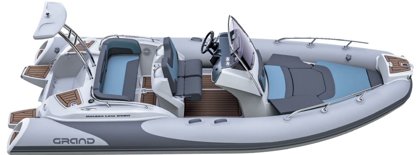
G580GLF with waterski towing arch with GRP top, sundecks and Mocha/Black SeaDek
